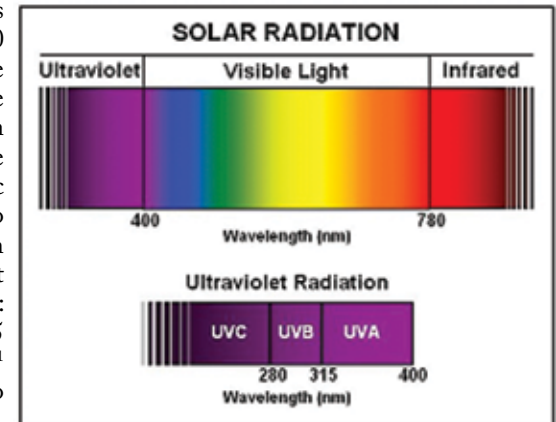
Figure 1. Electromagnetic radiation spectrum including visible, infrared, UVA, UVB, and UVC wavelengths.
